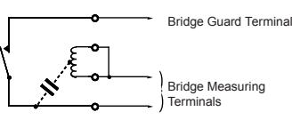
Measurement of C2- switch to coil
