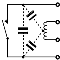
Measurement of C1- switch to coil
