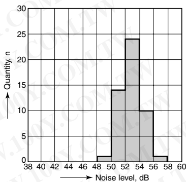
6.-(2)-1 Operation noise distribution (horizontal type)
