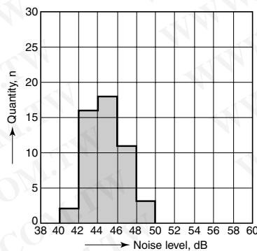
6.-(2)-2 Operation noise distribution (horizontal type)
