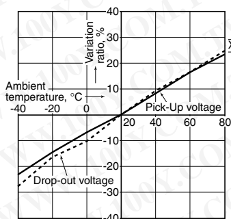
1. Ambient temperature characteristics 3 pcs.
