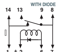
SPST - NC
