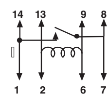
SPST - NO
