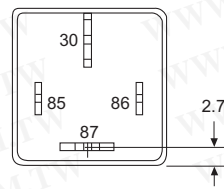
View of the terminals (bottom view)
