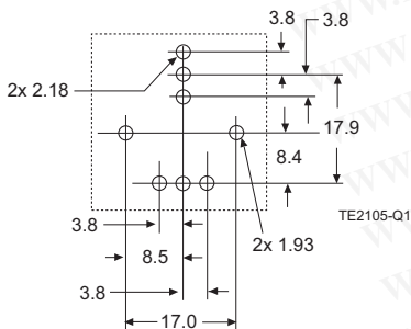
Bottom view on solder pins
