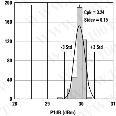
Figure 3. P1dB LSL = 28.5, Nominal = 30.
