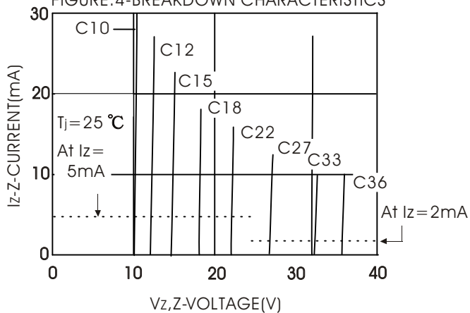
FIGURE.4-BREAKDOWN CHARACTERISTICS
