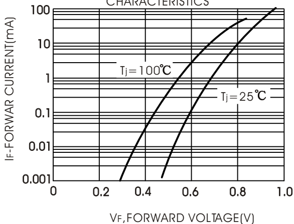
FIGURE.6-FORWARD CURRENT CHARACTERISTICS
