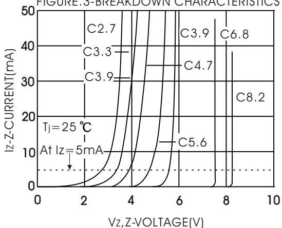
FIGURE.3-BREAKDOWN CHARACTERISTICS
