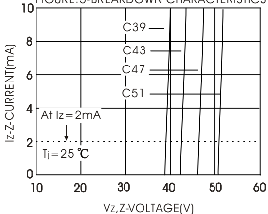
FIGURE.5-BREAKDOWN CHARACTERISTICS
