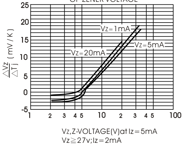
FIGURE. 13-TEMPERATURE DEPENDENCE OF ZENER VOLTAGE
