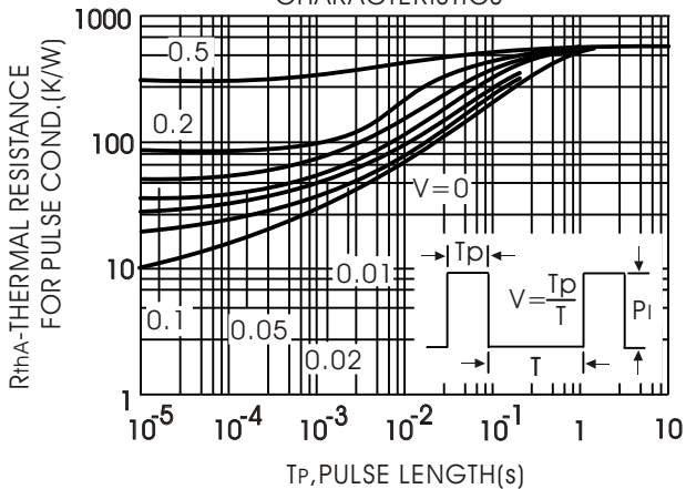
FIGURE.6-THERMAL RESISTANCE CHARACTERISTICS
