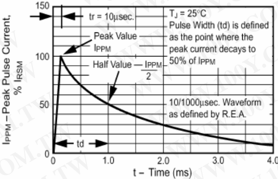
Fig. 3 – Pulse Waveform
