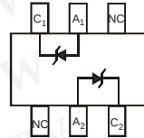
Device Schematic
