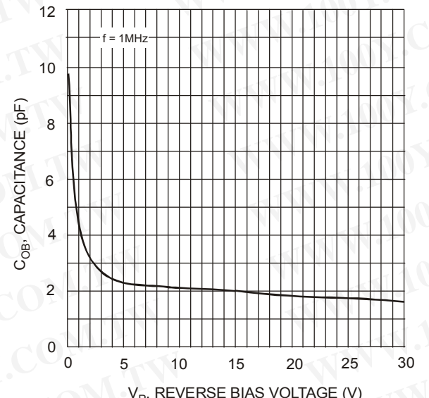
Fig. 4 Output Capacitance
