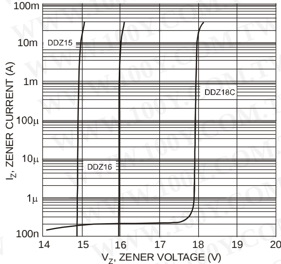
Fig. 6 Typical Zener Breakdown Characteristics, DDZ15 - DDZ18C
