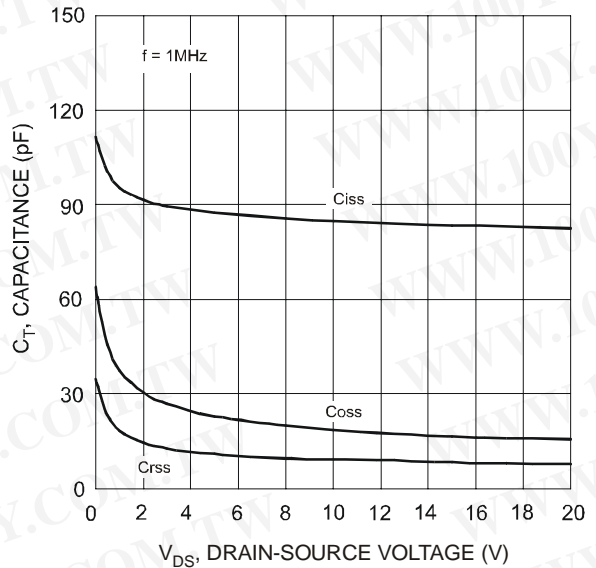
Fig. 10 Typical Capacitance
