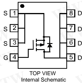
SOP-8L
