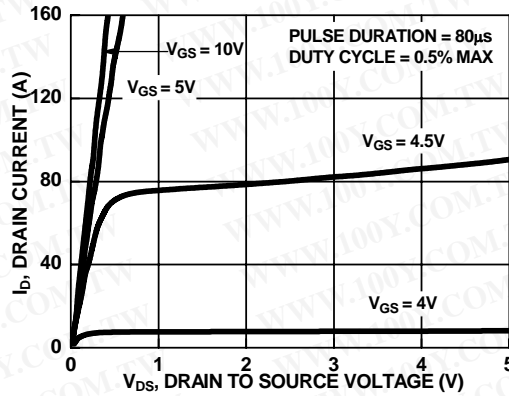
Figure 8. Saturation Characteristics
