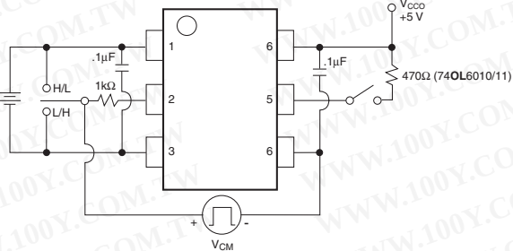
Figure 16. Common Mode Reiection Test Circuit
