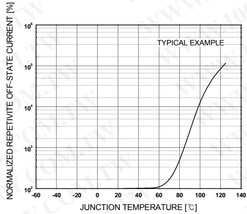
Figure 10. Repetitive Peak Off-state Current vs Junction Temperature
