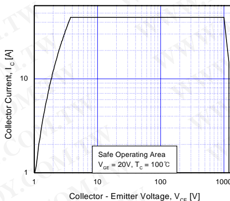
Fig 16. Turn-Off SOA
