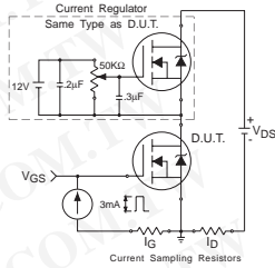
Fig 13a&b. Basic Gate Charge Test Circuit and Waveform
