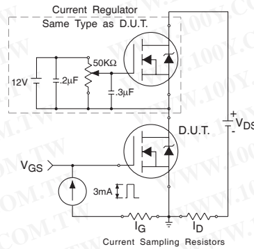
Fig 15. Gate Charge Test Circuit
