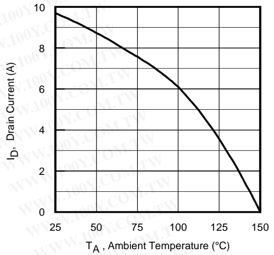
Fig 20. Maximum Drain Current vs. Ambient Temperature
