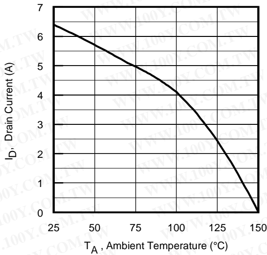
Fig 19. Maximum Drain Current vs. Ambient Temperature
