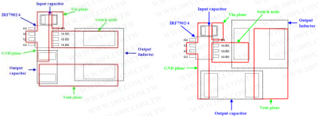
Fig 27. Layout Diagram
