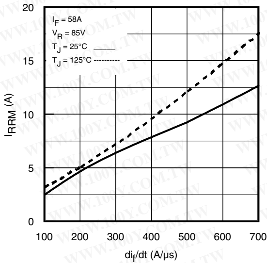
Fig. 18 - Typical Recovery Current vs. di_T/dt
