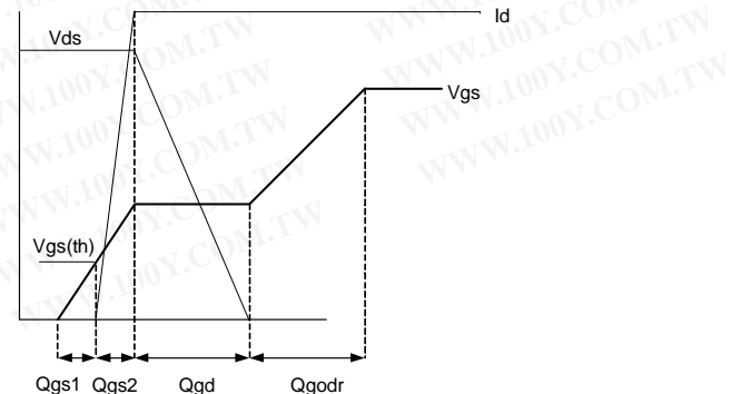
Fig 24b. Gate Charge Waveform
