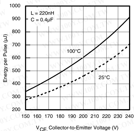
Fig 10. Typical E_{PULSE} vs. Collector-to-Emitter Voltage
