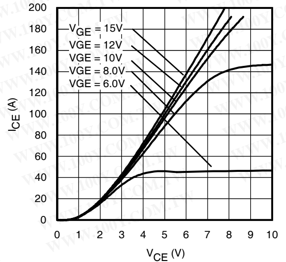
Fig. 6 - Typ. IGBT Output Characteristics T_J = 125^{\circ}C ; t_p = 80\mu s
