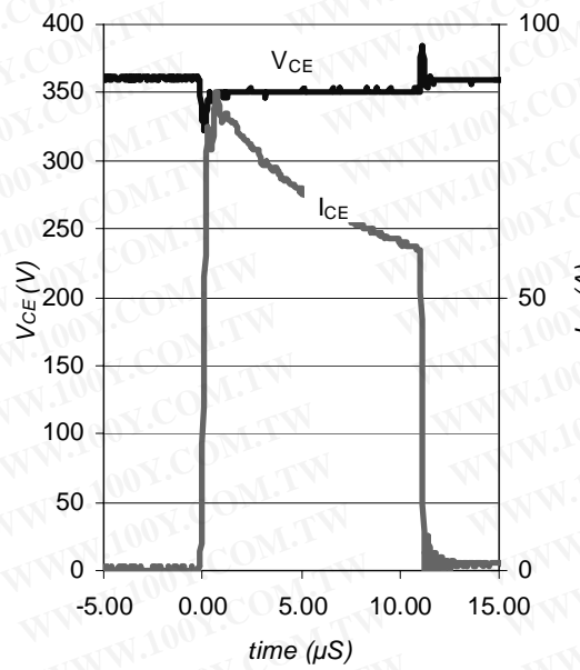
Fig. WF4- Typ. S.C Waveform @ T J = 150°C using Fig. CT.3
