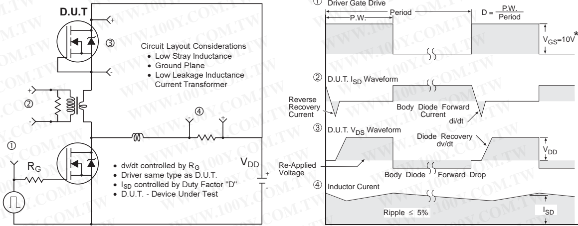
Fig 15. Peak Diode Recovery dv/dt Test Circuit for N-Channel HEXFET® Power MOSFETs
