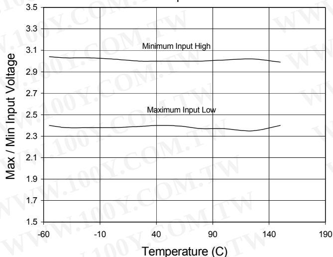
Fig. 10 Max / Min Input vs. Temperature CL = 1000 pF Vcc = 18V
