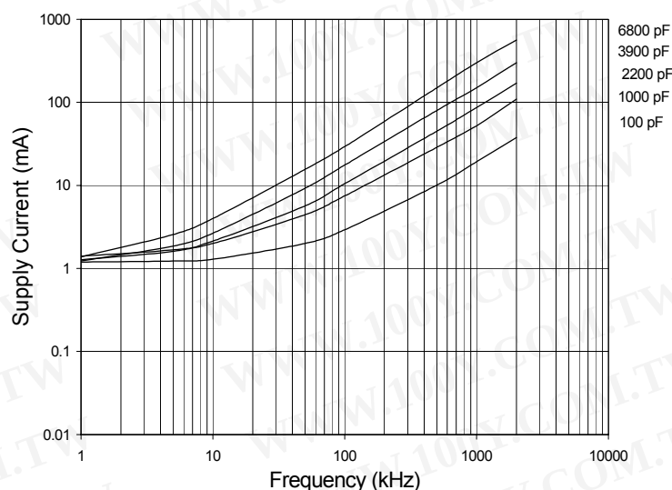
Supply Current vs. Frequency V_{CC} = 35V
