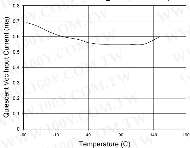
Quiescent Supply Current vs. Temperature V_{CC} = 18V , V_{in} = 5V @ 1kHz , CL = 1000\text{ pF}
