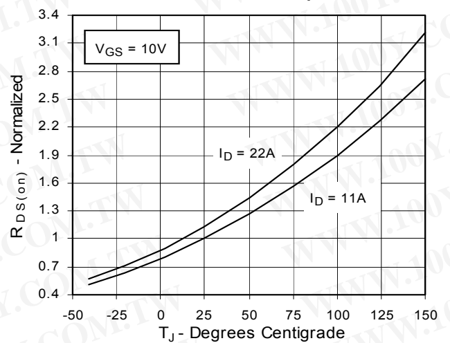
Fig. 4. R_{DS(on)} Normalized to I_D = 11A Value vs. Junction Temperature
