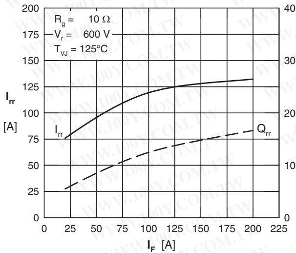
Fig. 11 Typ. reverse recovery characteristics
