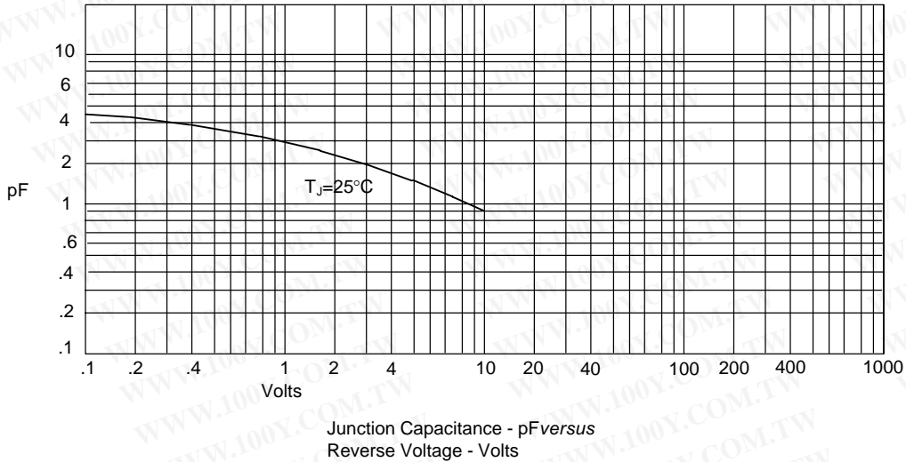
Figure 3 Junction Capacitance
