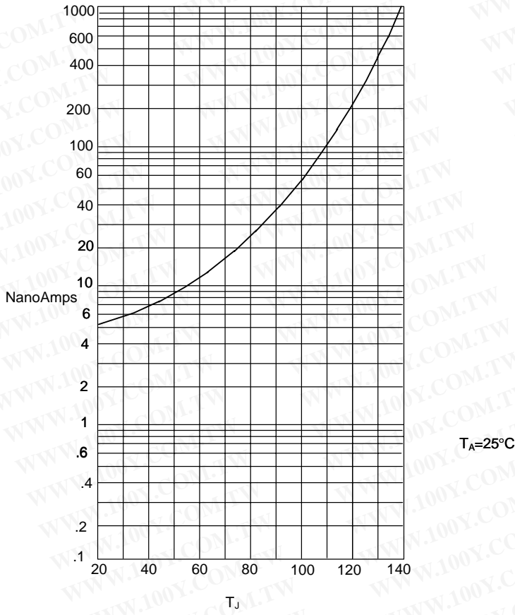
Instantaneous Reverse Leakage Current - NanoAmperes versus Junction Temperature - ^{\circ}C
