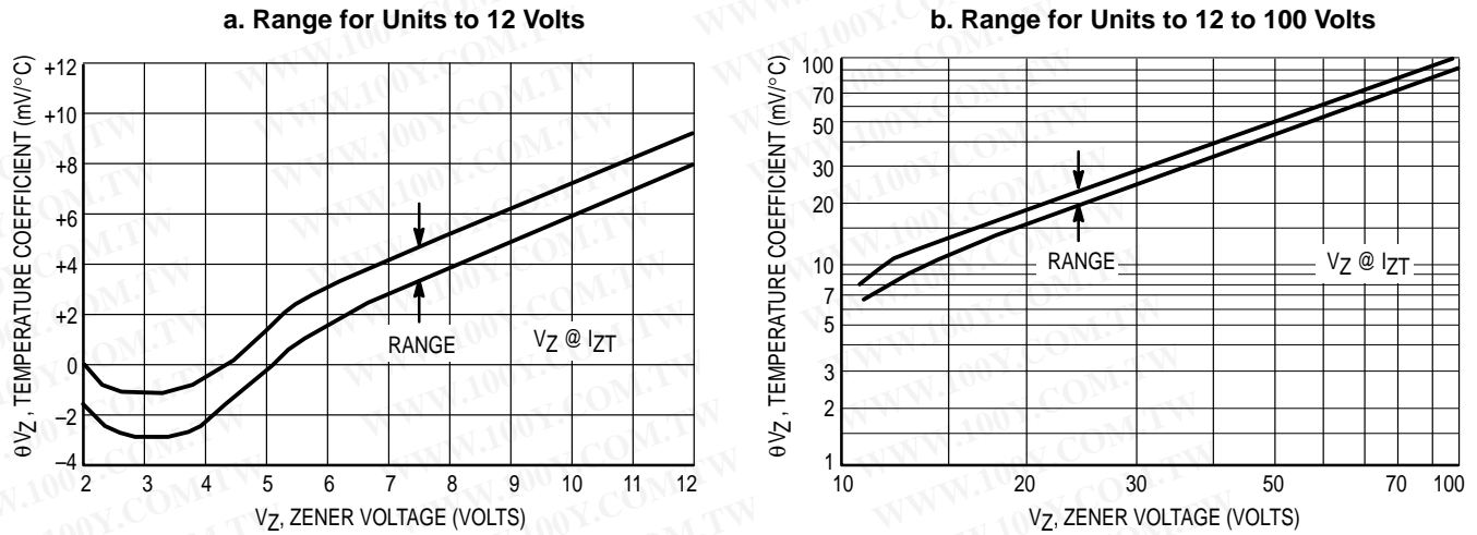
Figure 2. Temperature Coefficients
