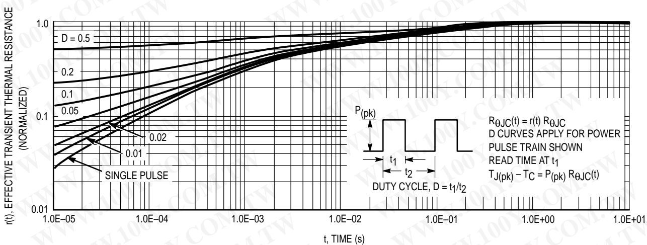
Figure 14. Thermal Response
