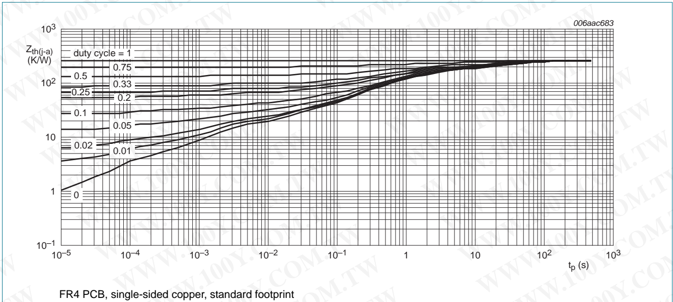
Fig 10. Transient thermal impedance from junction to ambient as a function of pulse duration for SOT1061; typical values
