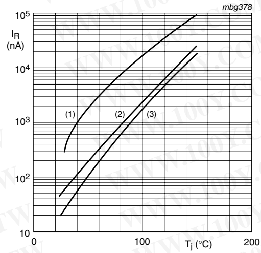
(1) V_R = 50\text{ V} ; maximum values (2) V_R = 30\text{ V} ; typical values (3) V_R = 50\text{ V} ; typical values
