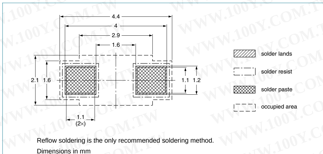
Fig 6. Reflow soldering footprint SOD123F
