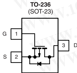
Top View Si2305DS (A5)* * Marking Code
