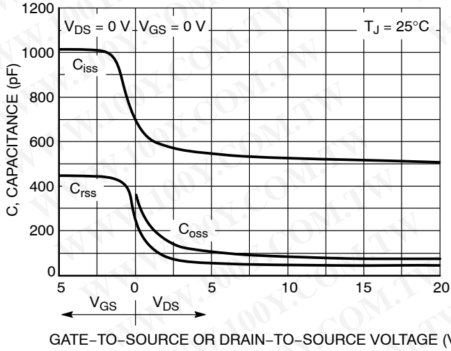
Figure 17. Capacitance Variation
