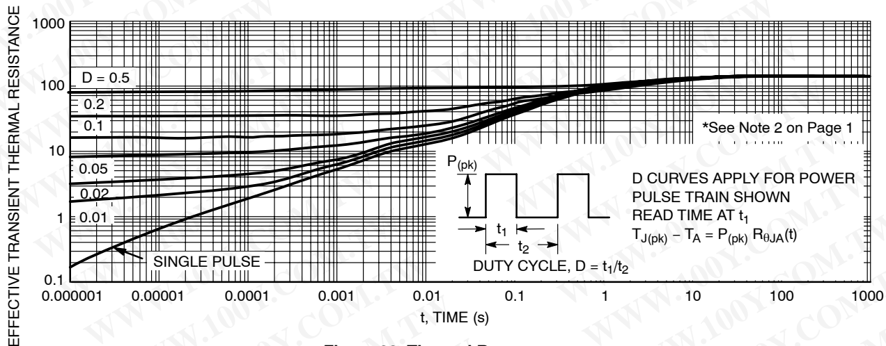
Figure 22. Thermal Response
