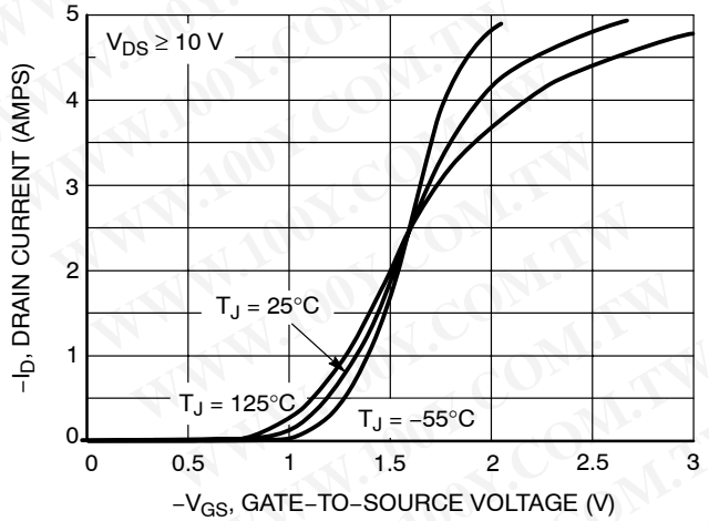
Figure 12. Transfer Characteristics
