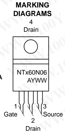
TO-220 CASE 221A STYLE 5
