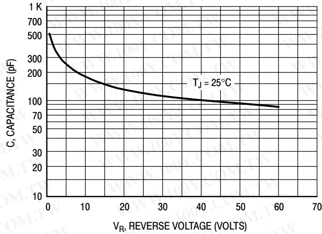
Figure 6. Typical Capacitance
