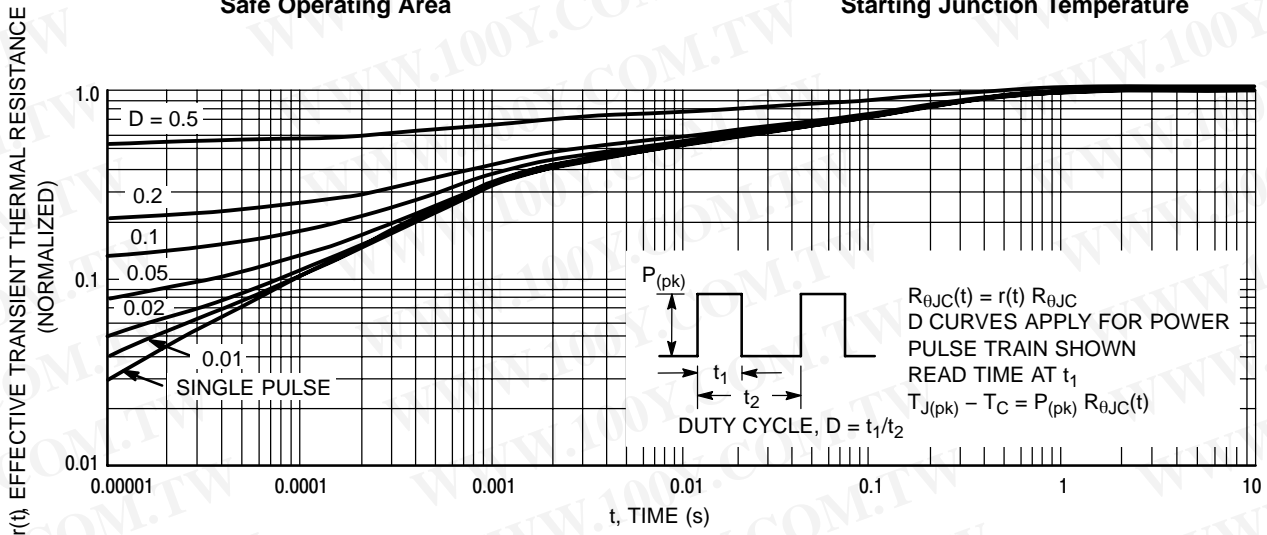
Figure 13. Thermal Response
