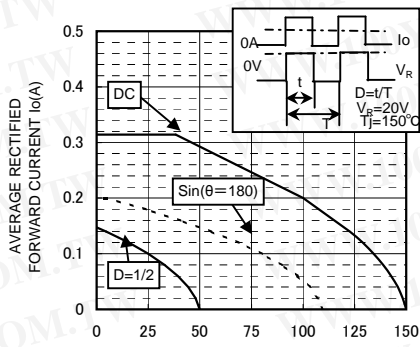
AMBIENT TEMPERATURE : T_a(^{\circ}C) Derating Curve*( I_o - T_a )
