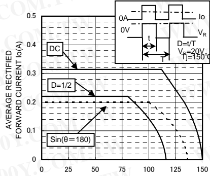
CASE TEMPERATURE : T_c(^{\circ}C) Derating Curve*( I_o - T_c )
