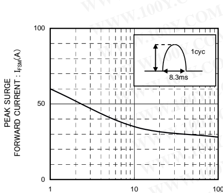
TIME : t (ms) I_{FSM} - t CHARACTERISTICS
