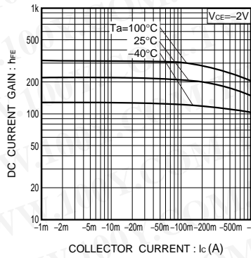
Fig.5 DC collector gain vs. collector current (II)
