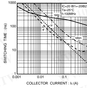
Fig.6 Switching time
