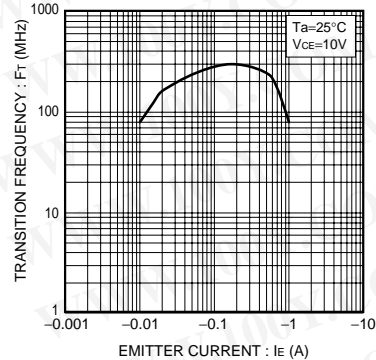
Fig.9 Transition frequency
