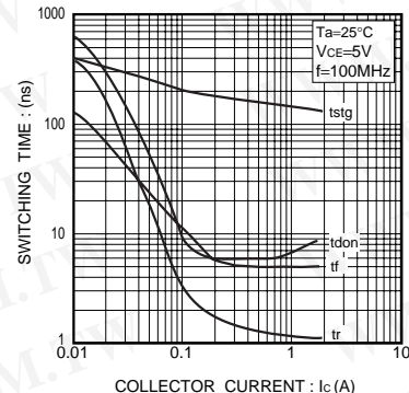
Fig.6 Switching time
