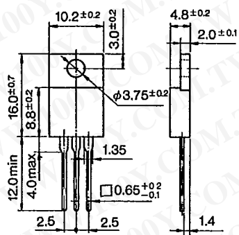
Outline Drawing Ⓔ
