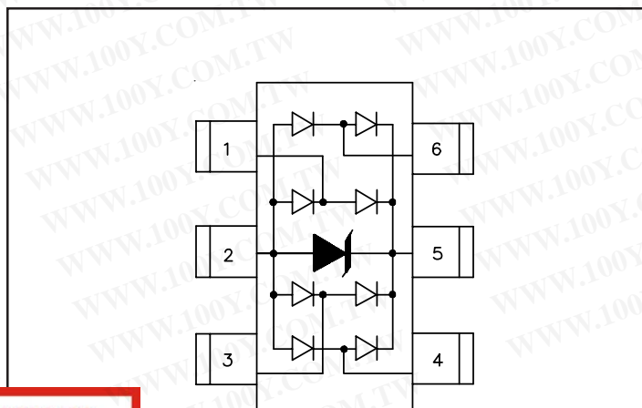
SOT-23 6L (Top View)
