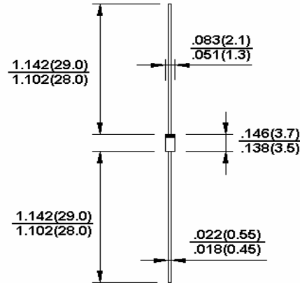
Dimensions is inches and (millimeters)
