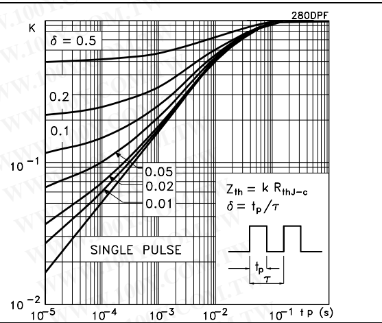
Figure 15. Thermal impedance for DPAK, IPAK
