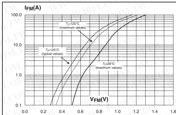
Figure 11. Forward voltage drop versus forward current (maximum values, per diode)
